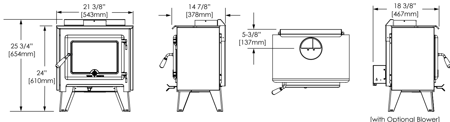
Figure 1: TN10 Dimensions.
